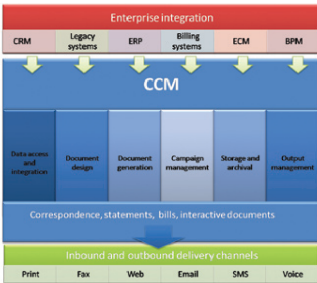
CCM Framework – Source: Quocirca
